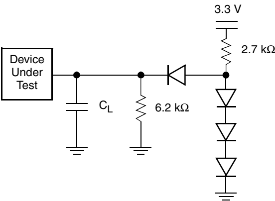
Figure 13. Test Setup
