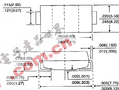
DO-214AB
