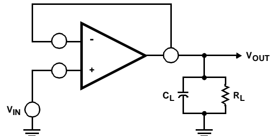
FIGURE 2. TRANSIENT RESPONSE TEST CIRCUIT FOR ALL TYPES
