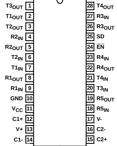
HIN211 (SOIC, SSOP) TOP VIEW
