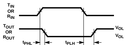
FIGURE 3. RECEIVER
