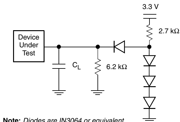
Figure 12. Test Setup
