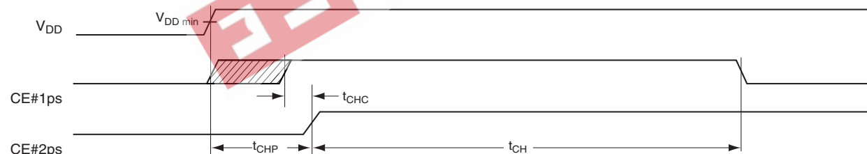
Figure 29. Power-on Timing
