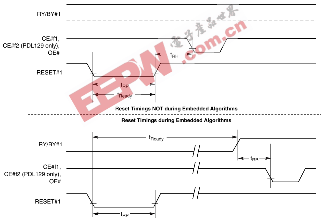
Figure 12. Reset Timings
