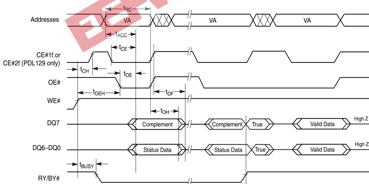
Figure 17. Data# Polling Timings (During Embedded Algorithms)
