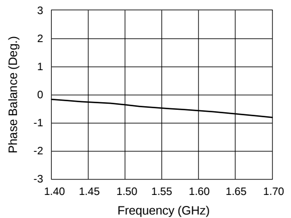
Phase Balance vs. Frequency
