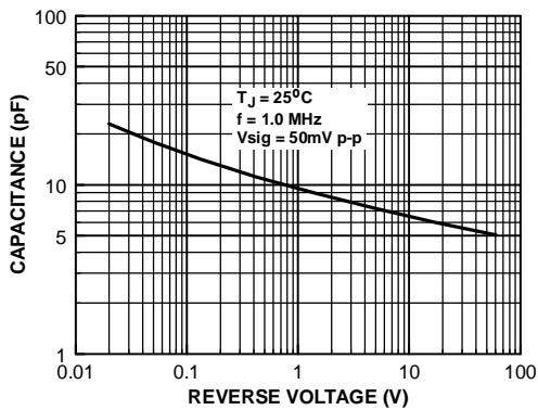
Junction Capacitance
