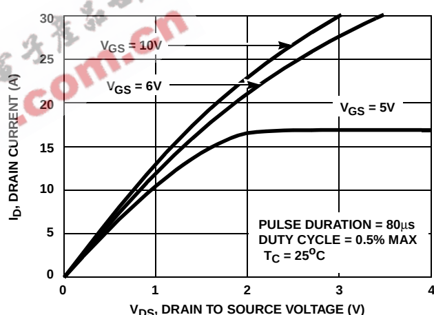
FIGURE 8. SATURATION CHARACTERISTICS
