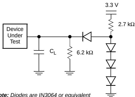
Figure 11. Test Setup
