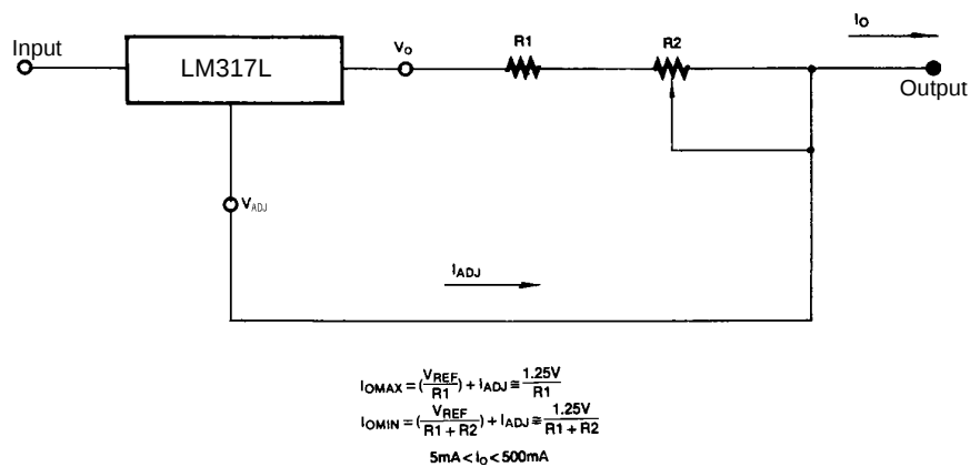
Figure 3. Current Regulator
