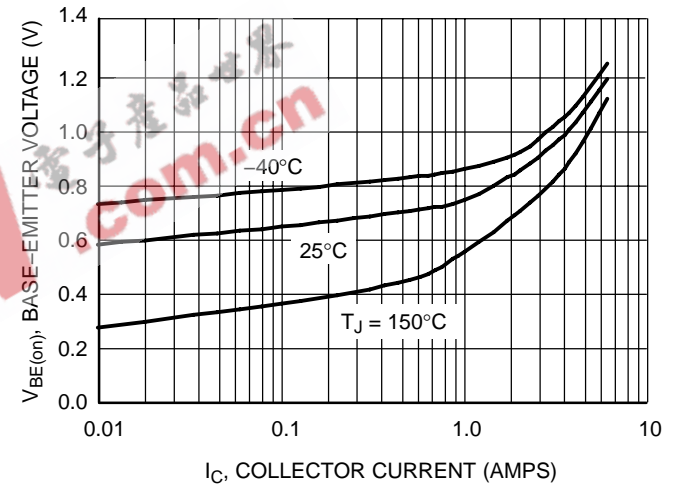
Figure 13. V_{BE(on)} PNP MJE15035
