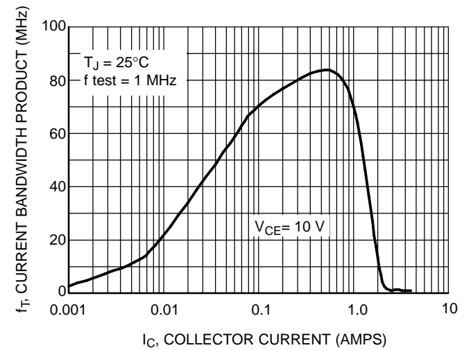
Figure 15. Typical Current Gain Bandwidth Product PNP MJE15035
