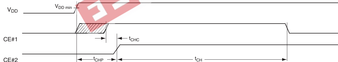
Figure 34. Power-on Timing
