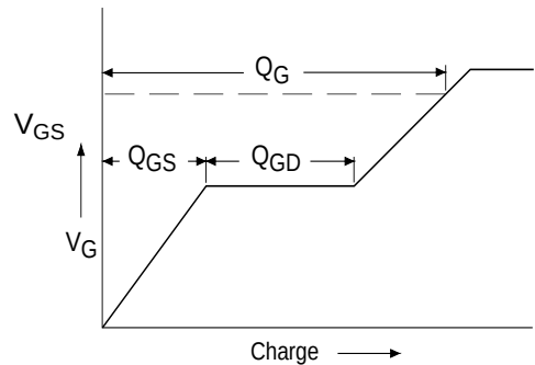
Fig 13b. Basic Gate Charge Waveform
