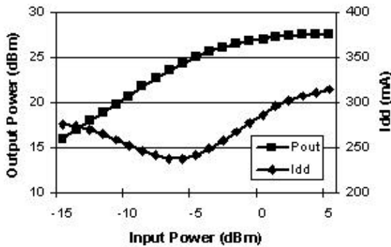
Output Power and Drain Current vs. Input Power, T_s = +37\text{ }^\circ\text{C}
