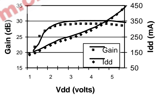
Gain and Drain Current vs. Voltage, T_s = +37\text{ }^\circ\text{C}
