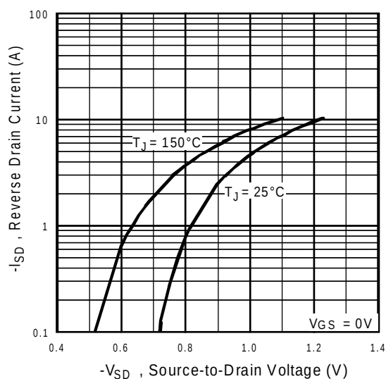
Fig 4. Typical Source-Drain Diode Forward Voltage
