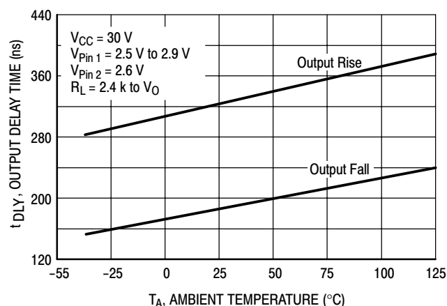
Figure 7. Uncommitted Comparator Delay versus Temperature
