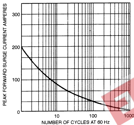
FIG. 1-MAXIMUM NON-REPETITIVE PEAK FORWARD SURGE CURRENT - PER ELEMENT
