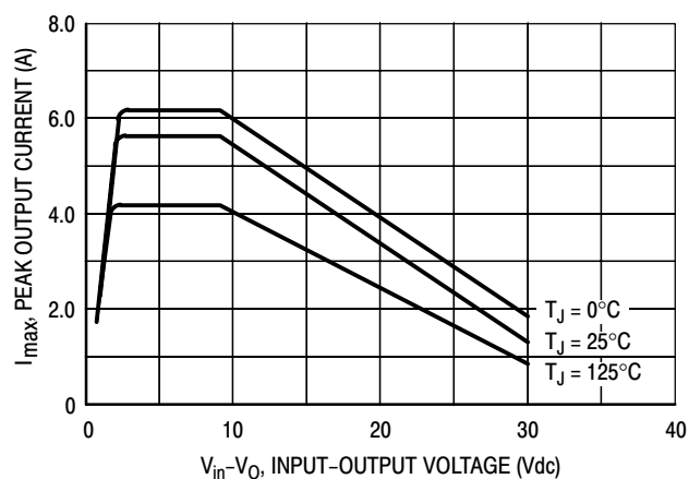
Figure 11. Peak Output Current
