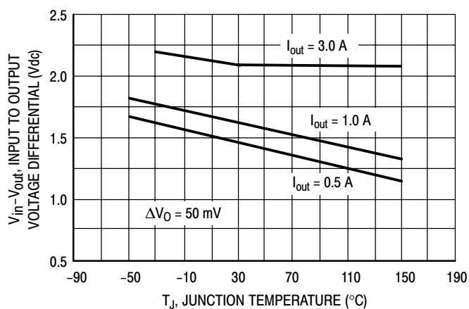
Figure 10. Dropout Voltage
