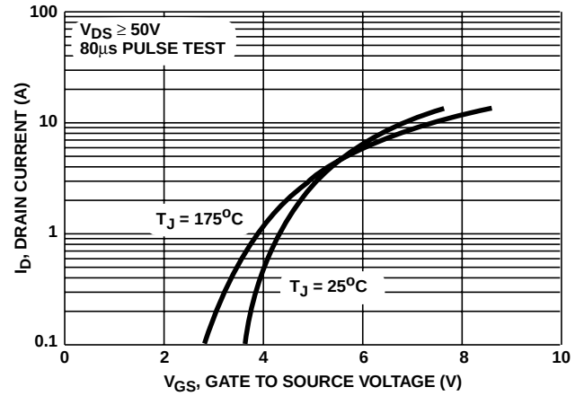
FIGURE 7. TRANSFER CHARACTERISTICS
