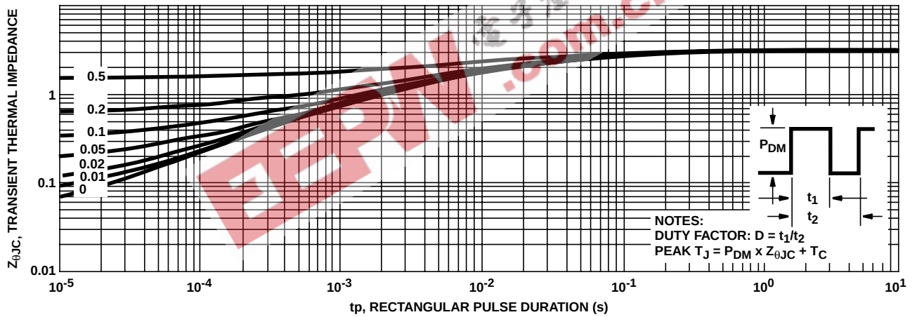
FIGURE 20. MAXIMUM TRANSIENT THERMAL IMPEDANCE
