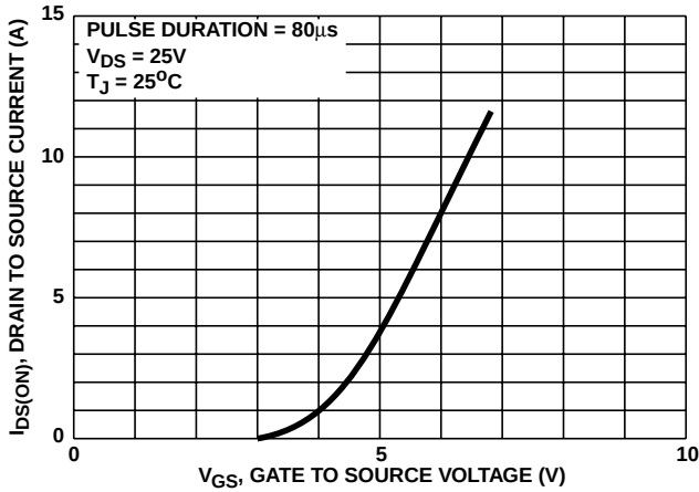
FIGURE 23. TRANSFER CHARACTERISTICS
