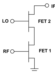
Figure 17. Cascode FET Mixer.
