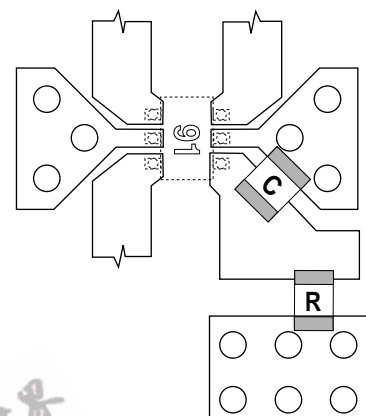
Figure 21. RFLayout.
