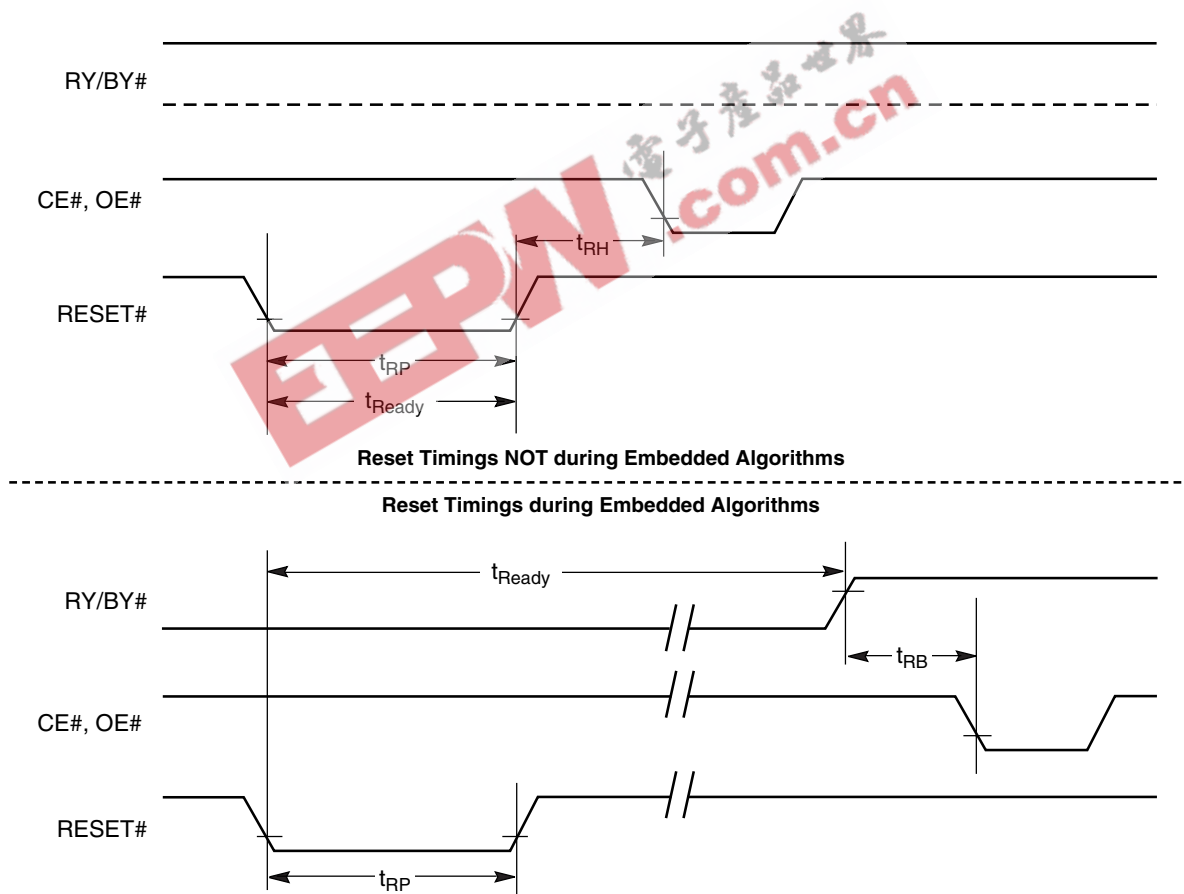
Figure 16. Reset Timings
