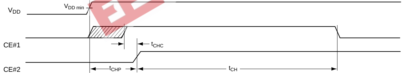
Figure 34. Power-on Timing
