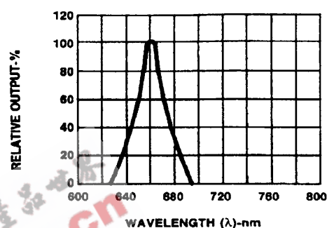
Fig.2 SPECTRAL RESPONSE
