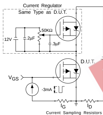
Fig 9b. Gate Charge Test Circuit
