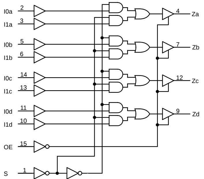
Figure 2. Logic Diagram
