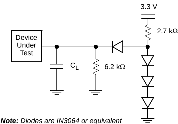
Figure 11. Test Setup
