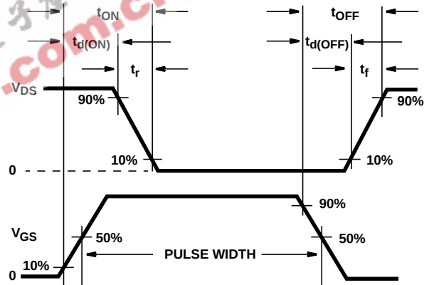
FIGURE 15. RESISTIVE SWITCHING WAVEFORMS
