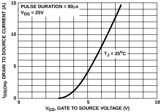
FIGURE 6. TRANSFER CHARACTERISTICS
