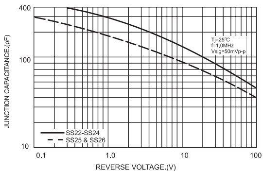
FIG.5-TYPICAL JUNCTION CAPACITANCE
