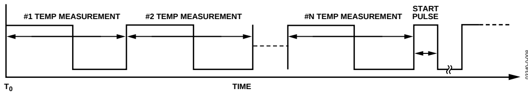
Figure 28. Daisy-Chain Signal at Input to the Microcontroller
