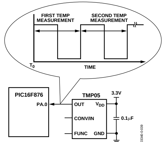
Figure 37. Typical Daisy-Chain Application Circuit
