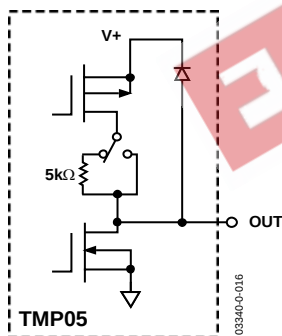
Figure 24. TMP05 One Shot Mode OUT Pin Configuration
