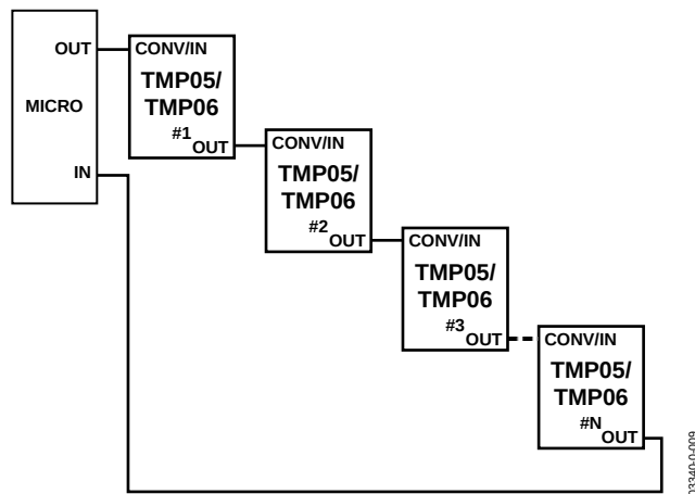
Figure 25. Daisy-Chain Structure
