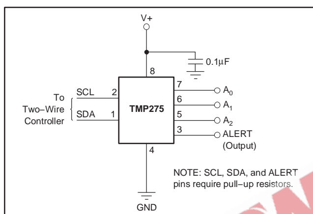
Figure 1. Typical Connections of the TMP275
