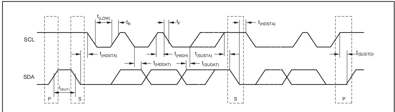
Figure 4. Two-Wire Timing Diagram
