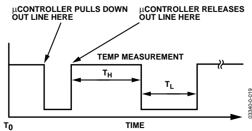
Figure 23. TMP05/TMP06 One Shot OUT Pin Signal
