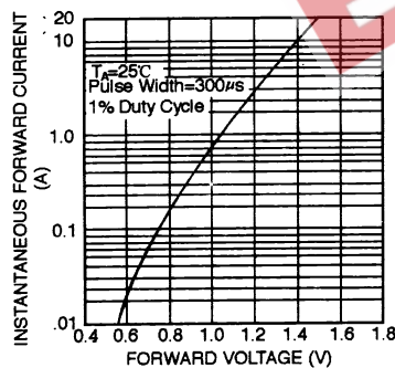
FIG.3-TYPICAL FORWARD CHARACTERISTICS
