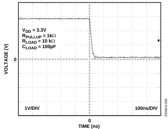
Figure 11. TMP06 Output Fall Time at 25^{\circ}C
