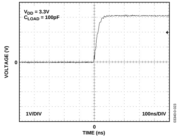
Figure 9. TMP05 Output Rise Time at 25^{\circ}C
