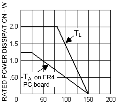
T_L , LEAD TEMP. ( ^{\circ} C) or T_A on FR4 PC Board
