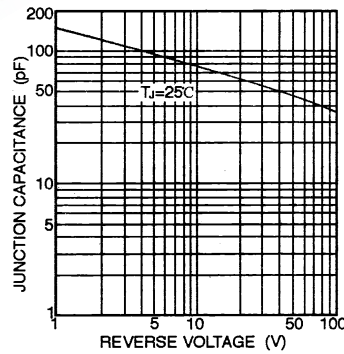
FIG. 4-TYPICAL JUNCTION CAPACITANCE
