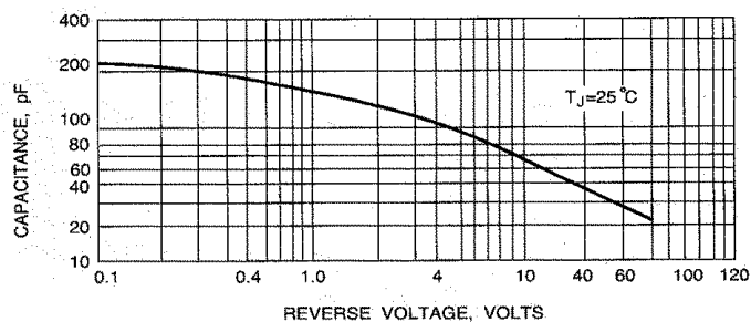
Fig. 4 - TYPICAL JUNCTION CAPACITANCE
