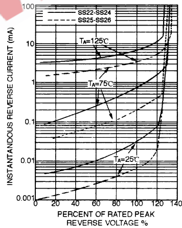
FIG. 4 – TYPICAL REVERSE CURRENT CHARACTERISTICS
