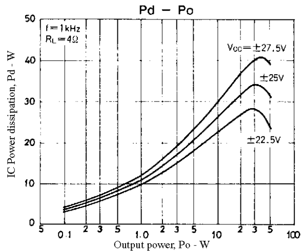
Figure 2. STK4028V Pd - Po ( R_L = 4\Omega )
