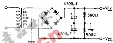
Specified Transformer Power Supply (Equivalent to RP-25)
