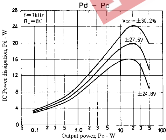
Figure 1. STK4028V Pd - Po ( R_L = 8\Omega )
