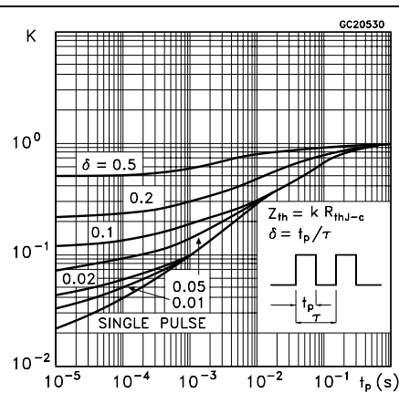
Figure 2. Thermal impedance for TO-220/ D 2 PAK/I 2 PAK
