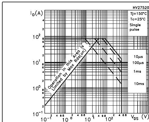
Figure 1. Safe operating area for TO-220/ D 2 PAK/I 2 PAK
