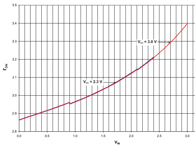
Figure 5. r_{ON} ( I_{OUT} = -30 mA)
