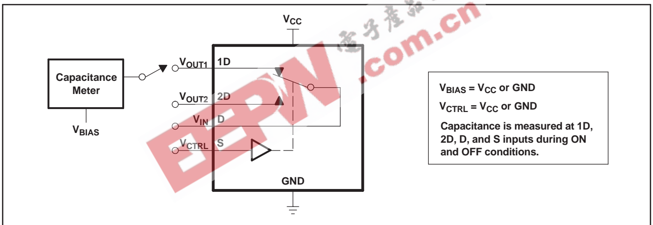
Figure 17. Capacitance
