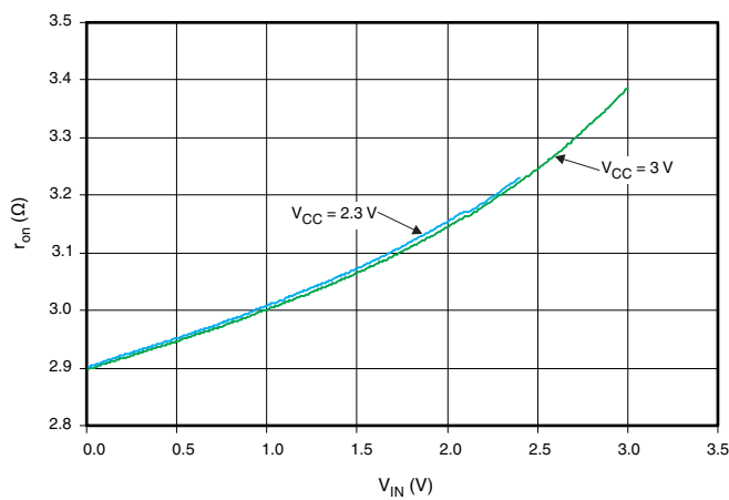
Figure 5. r_{ON} vs V_{IN} ( I_{OUT} = 30 mA)
