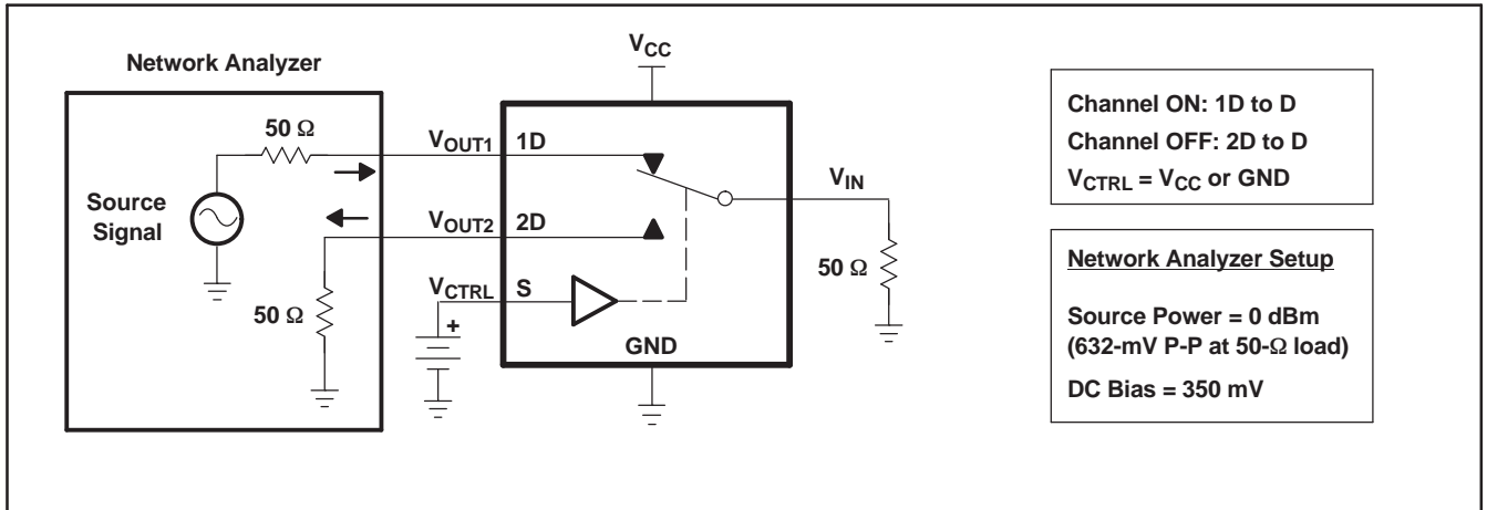
Figure 11. Crosstalk (X TALK )
