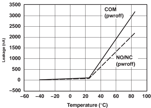
Figure 5. Leakage Current vs Temperature
