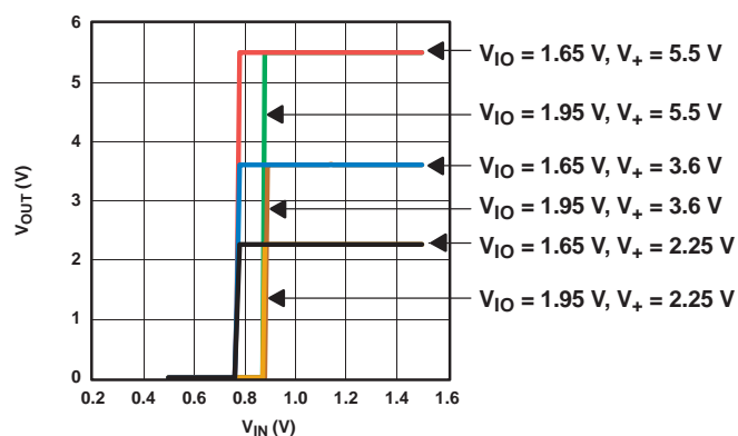
Figure 13. V_{IO} Thresholds
