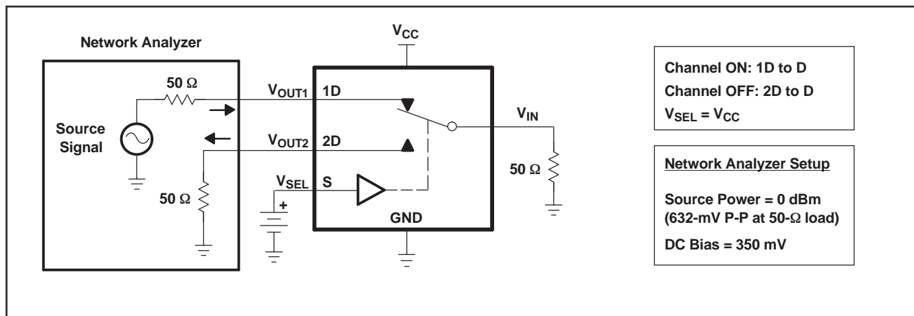
Figure 10. Crosstalk ( X_{TALK} )
