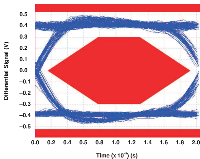
Figure 7. Eye Pattern: 480-Mbps USB Signal With Switch NC Path
