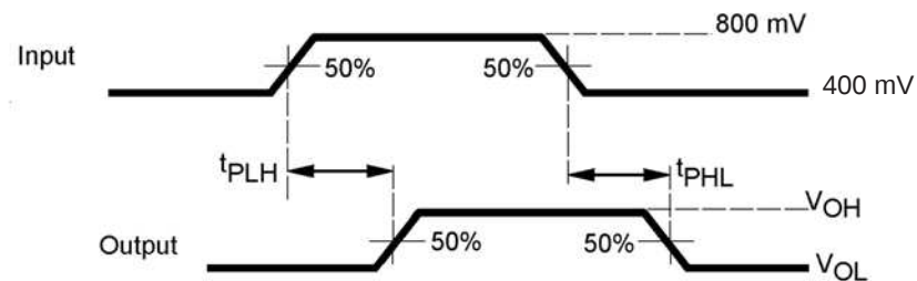
Figure 13. Propagation Delay
