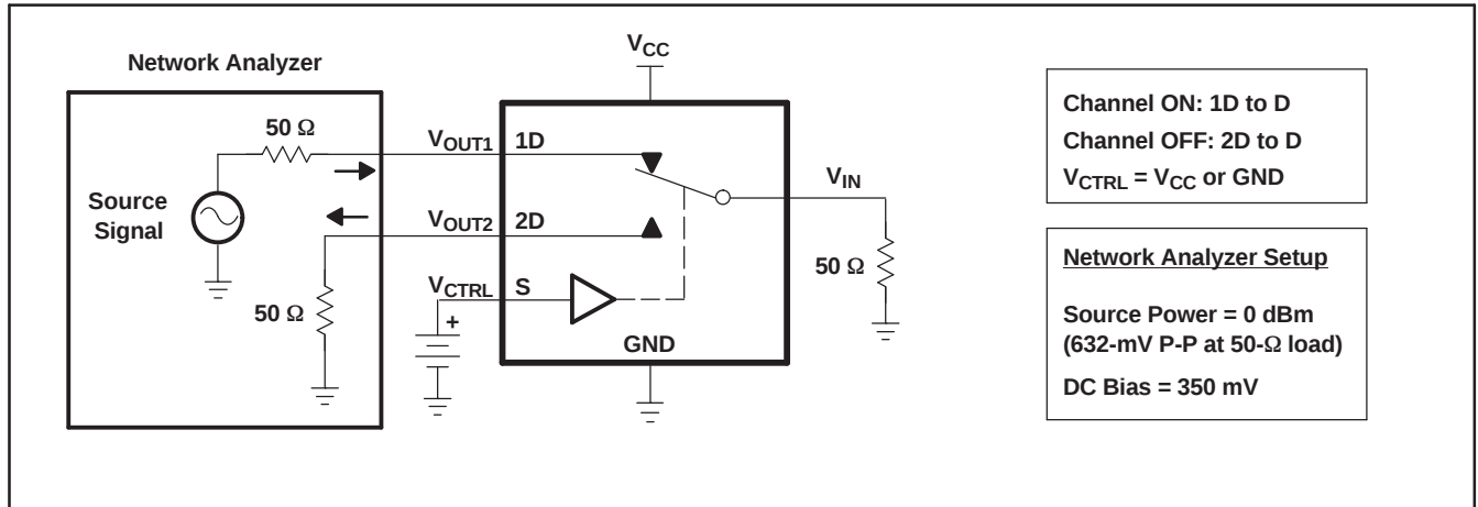
Figure 11. Crosstalk ( X_{TALK} )
