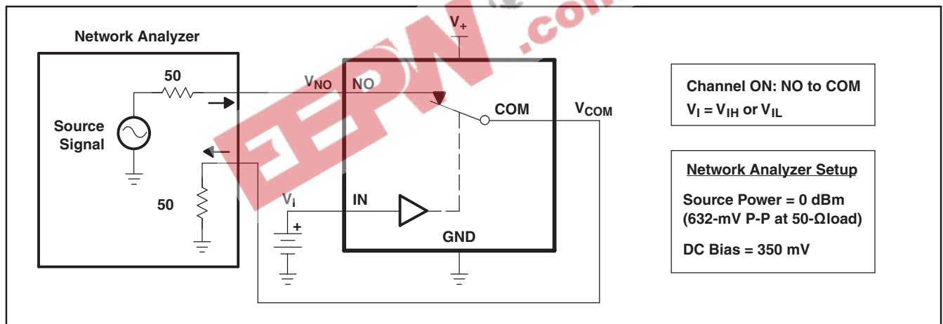
Figure 20. Bandwidth (BW)
