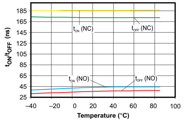
Figure 8. t_{ON}/t_{OFF} vs Temperature
