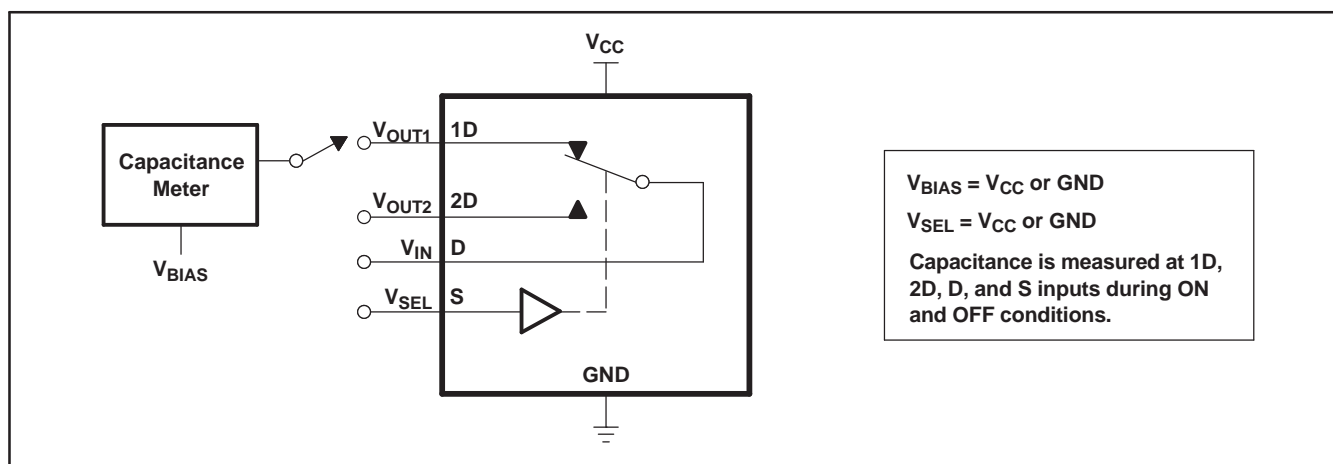
Figure 13. Capacitance
