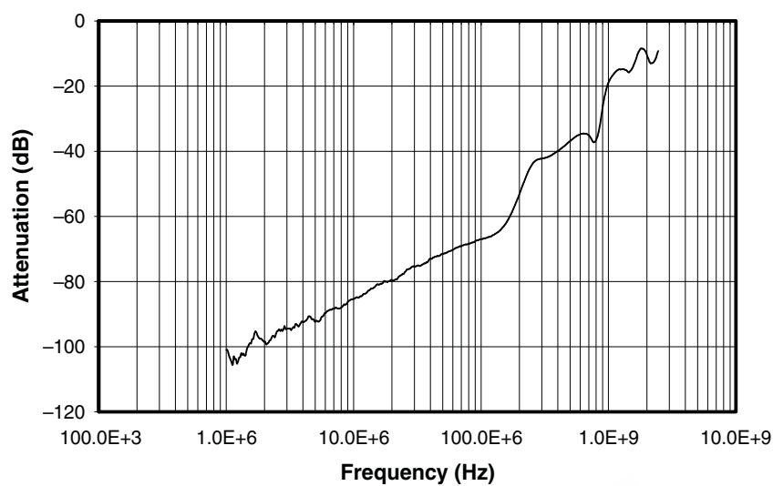
Figure 3. Crosstalk
