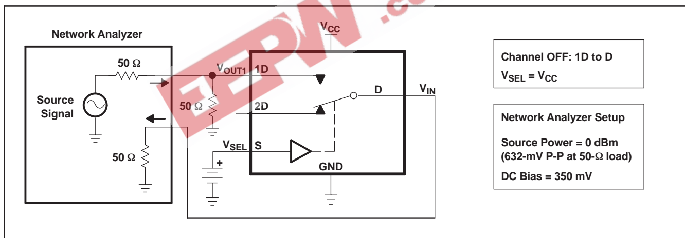
Figure 6. OFF Isolation ( O_{IRR} )
