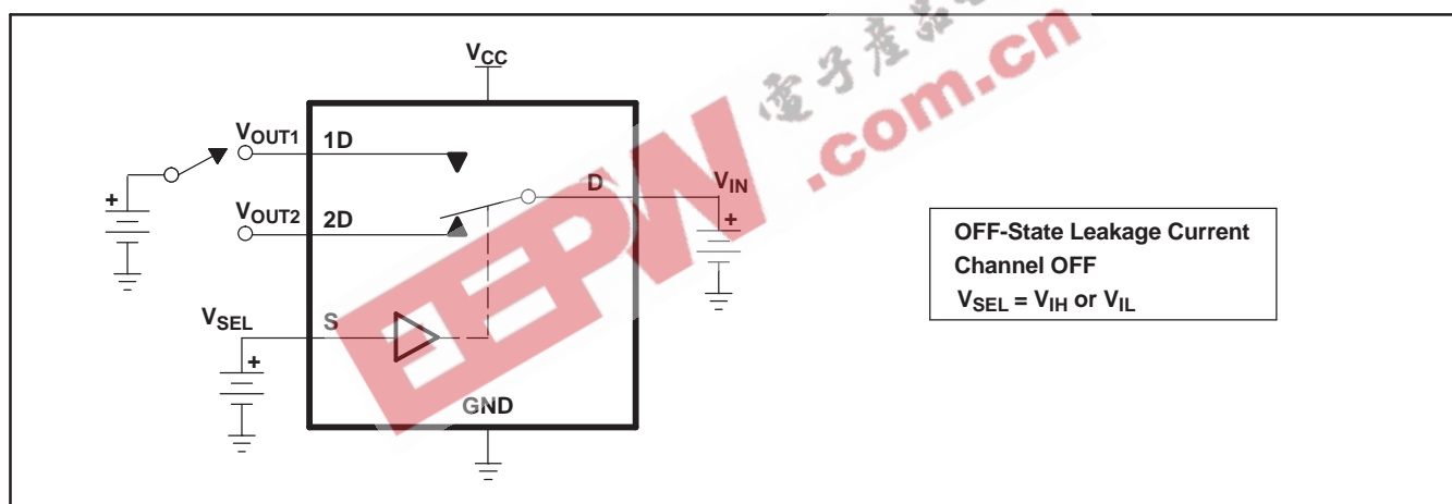
Figure 12. OFF-State Leakage Current
