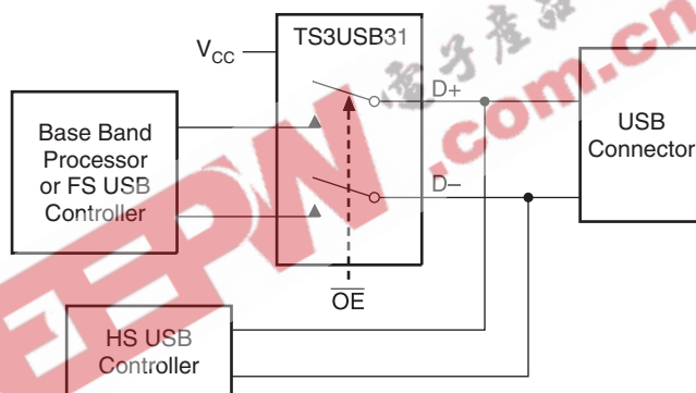
Figure 4. Application Diagram
