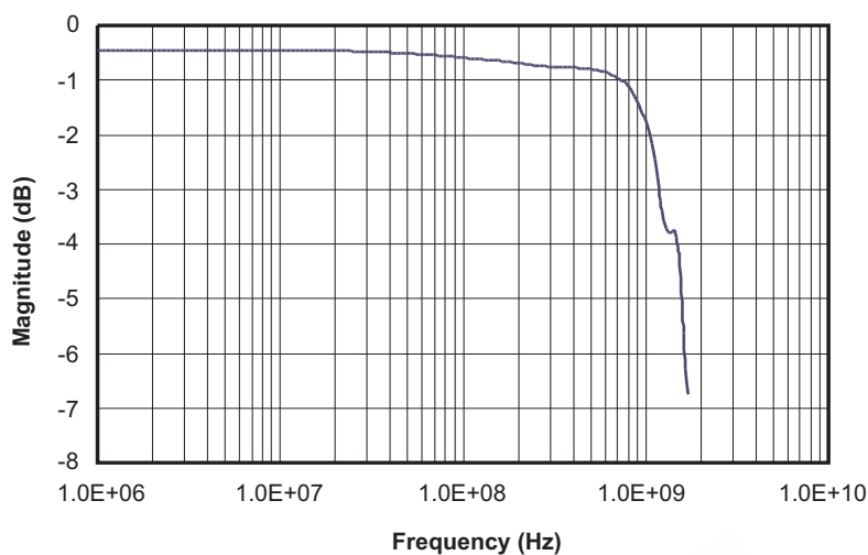
Figure 1. Insertion Loss
