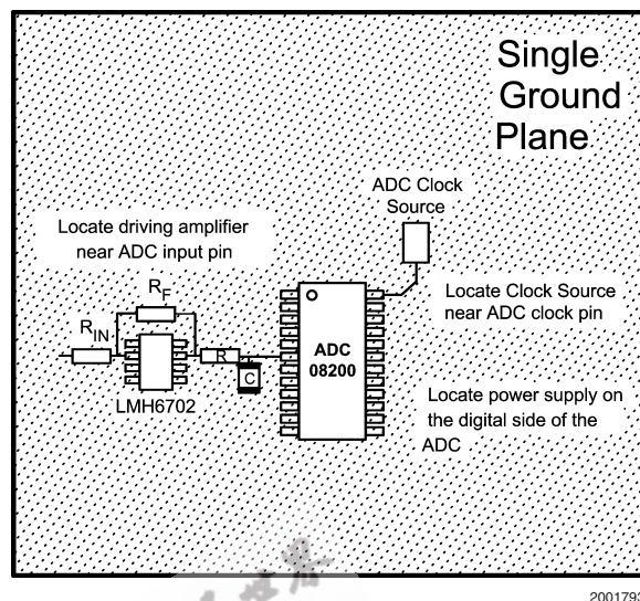
FIGURE 5. Layout Example
