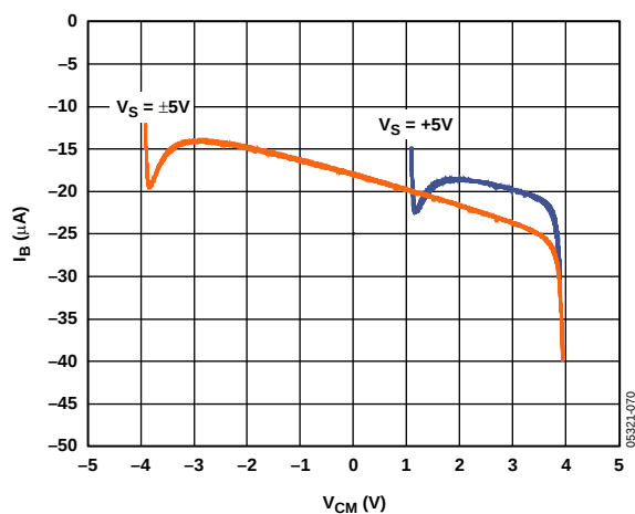
Figure 44. Input Bias Current vs. Common-Mode Voltage
