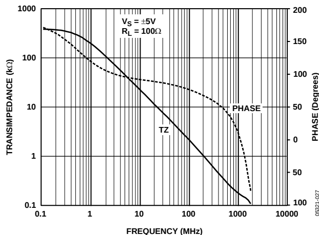
Figure 10. Transimpedance and Phase vs. Frequency
