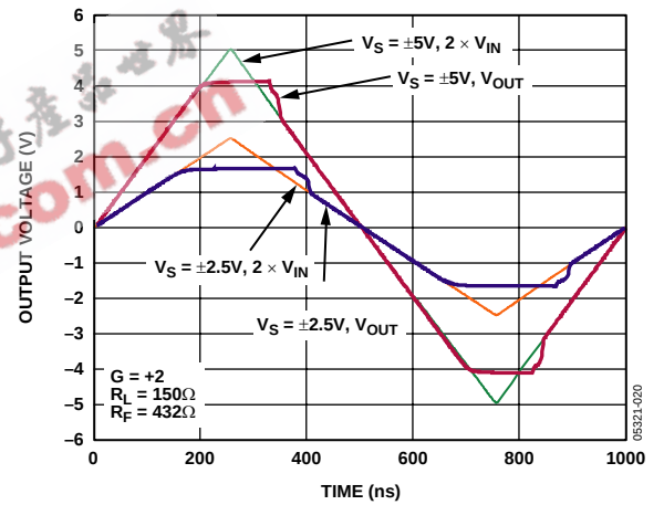
Figure 39. Output Overdrive
