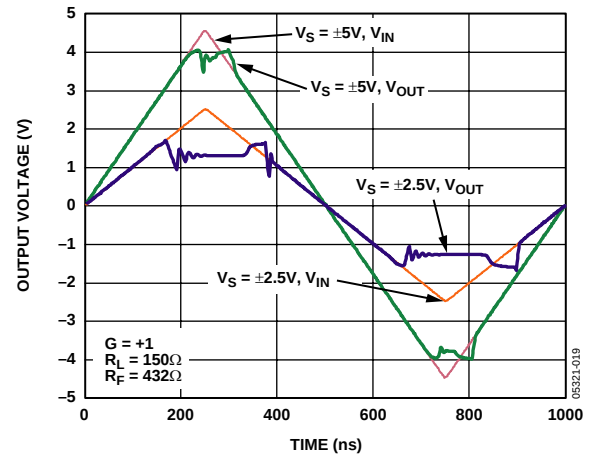
Figure 38. Input Overdrive
