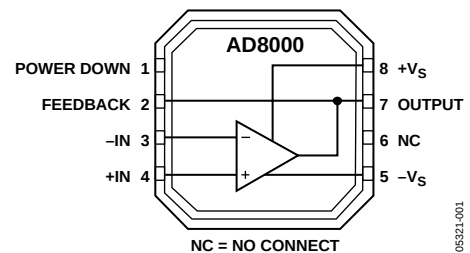
Figure 1. 8-Lead AD8000, 3 mm x 3 mm LFCSP (CP-8-2)
