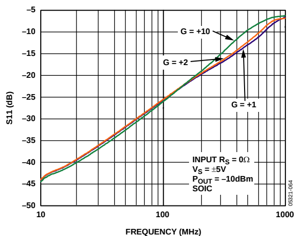
Figure 46. Input Voltage Standing Wave Ratio (S11)
