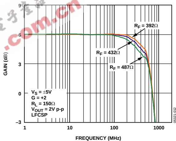
Figure 9. Large Signal Frequency Response vs. R_F
