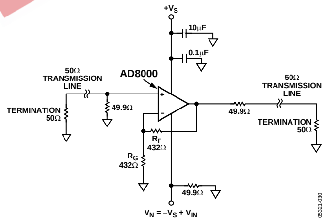
Figure 49. Negative PSRR
