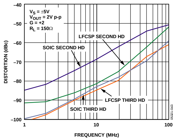
Figure 22. Harmonic Distortion vs. Frequency
