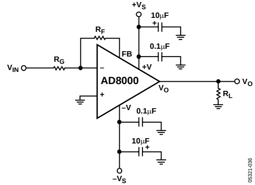
Figure 51. Inverting Configuration
