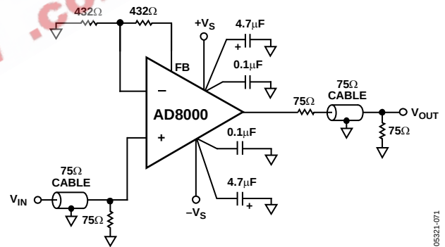
Figure 52. Video Line Driver
